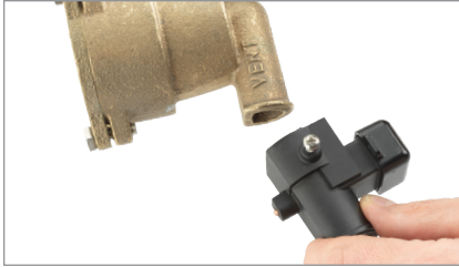
1. Position the flood sensor on the relief valve.
